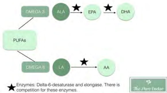
Figure 2: Schema of formation of omega-3 fatty acids from ALA and of omega-6 fatty acids (LA = linoleic acid; AA=arachidonic acid).
