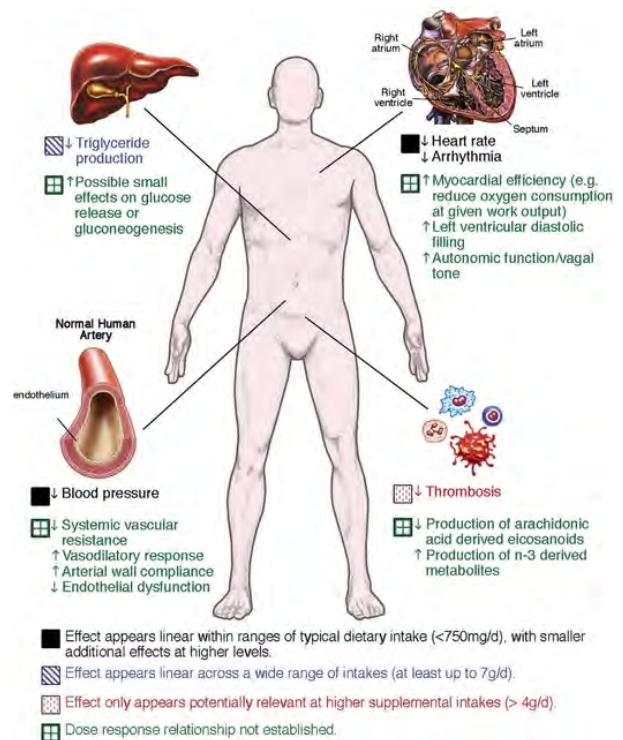
Figure 3: Potential factors in relation to omega-3 FAs and cardiovascular health.
